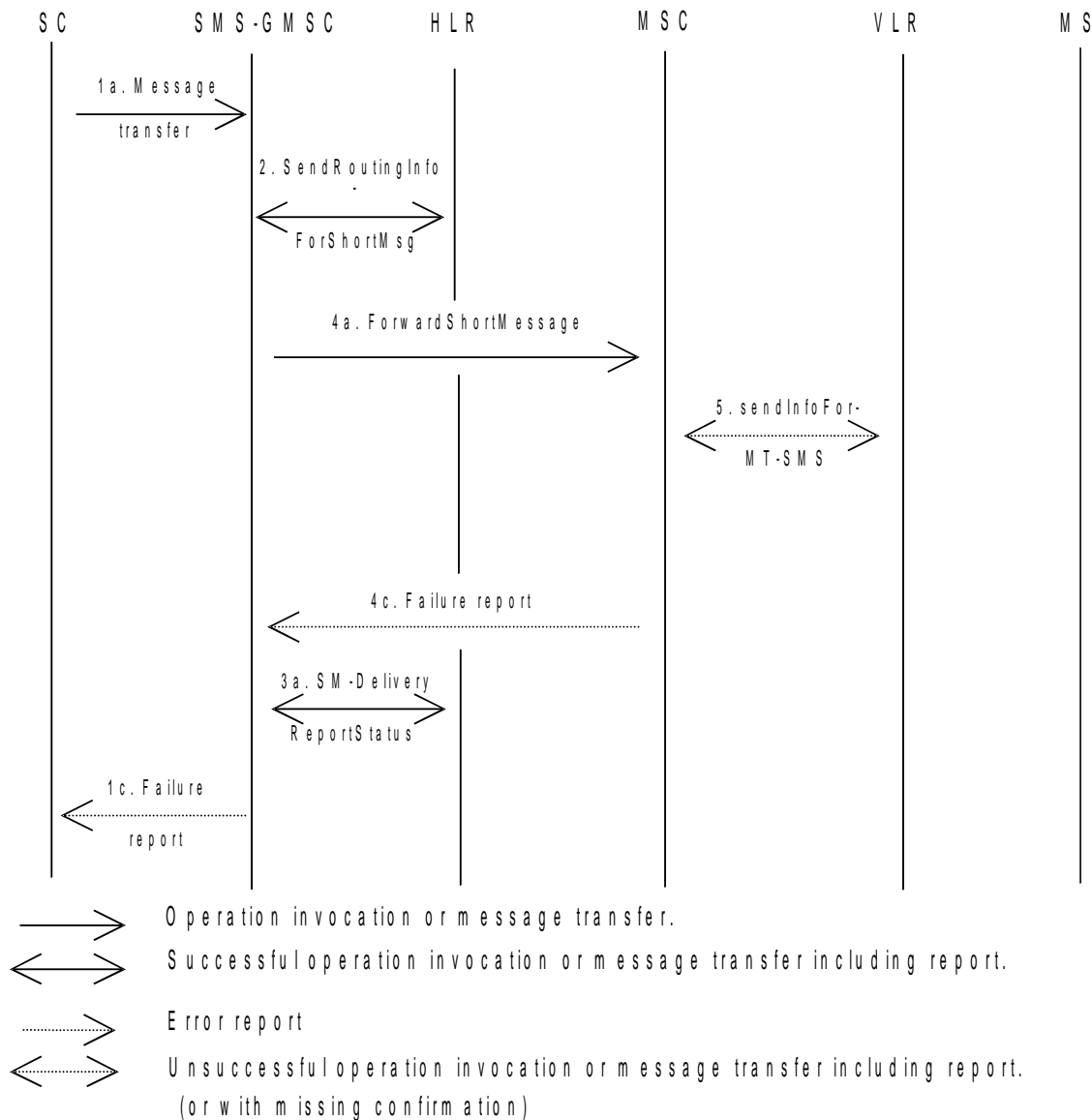
Figure 03.40/15e): Short message transfer attempt failing due to negative outcome of VLR information retrieval
