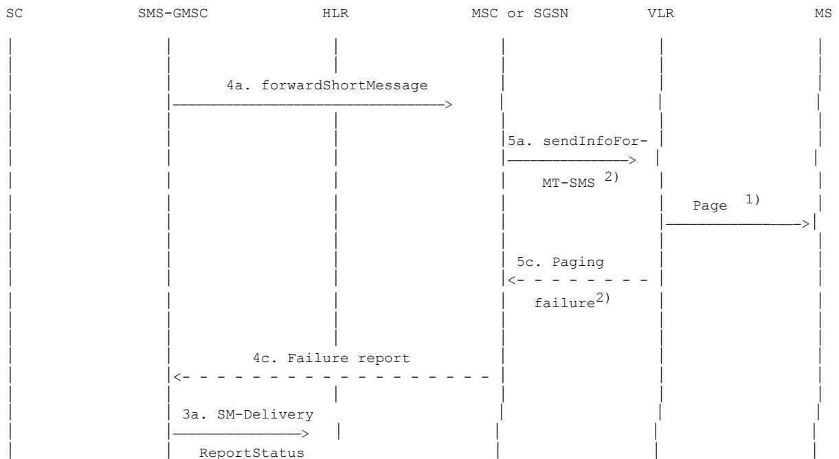
Figure 03.40/16b): "Send information for MT SMS" procedure; erroneous case: absent subscriber (e.g. IMSI DETACH or GPRS DETACH)
